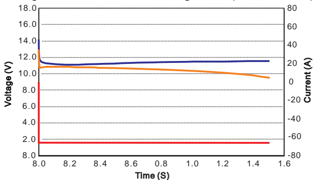
Voltage Vs Time Vs Current Discharge Curve (10 C, 90S, -10°C)
