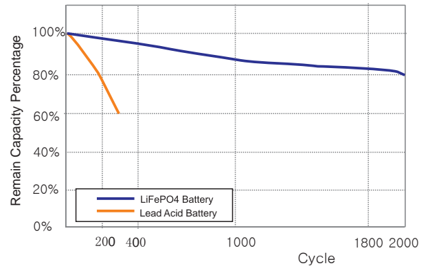
Cycle Life Performance Curve@25°C
